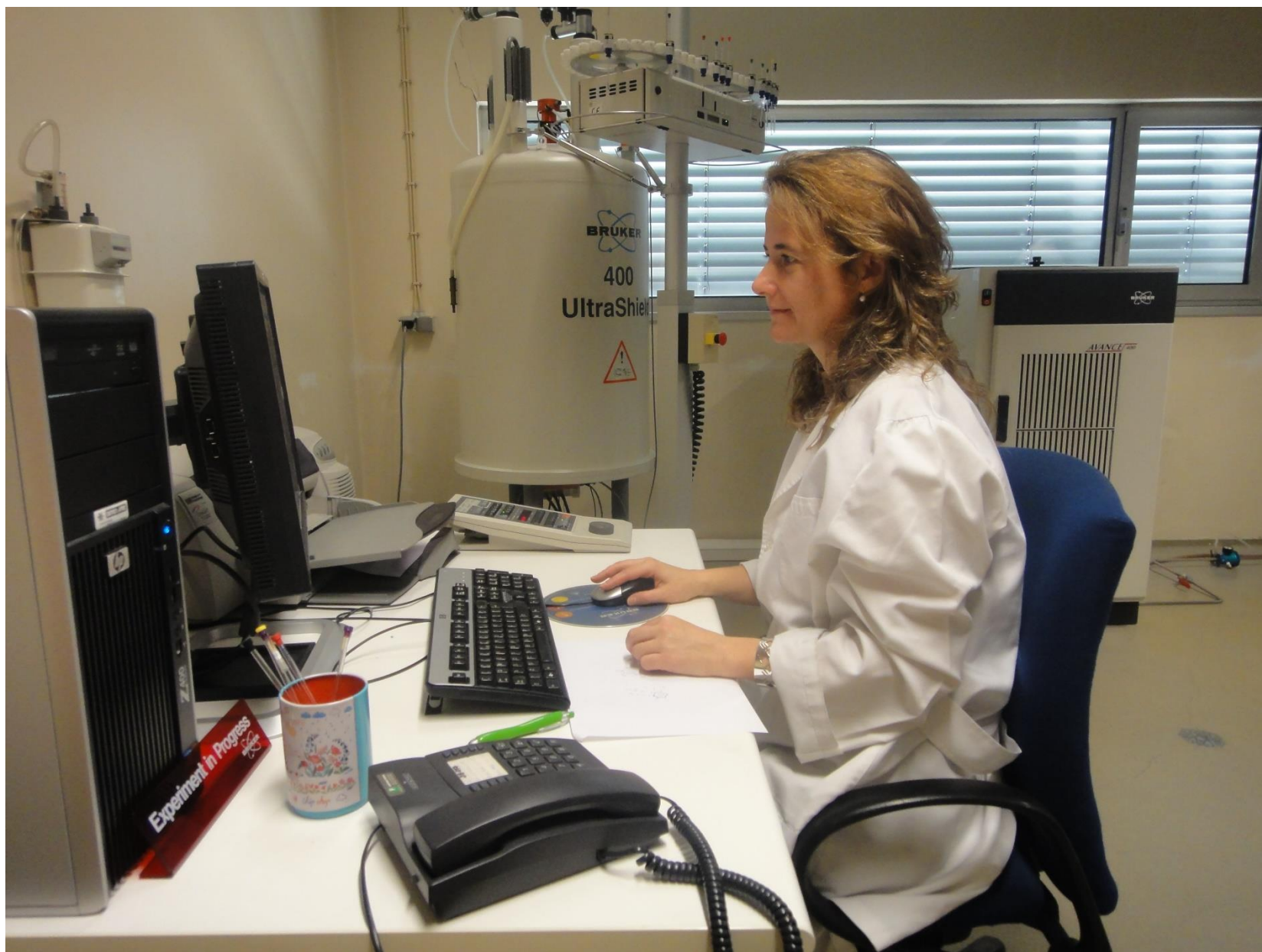
Nuclear magnetic resonance - RMN
